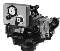
255 Series 3/4 Inch Valve Body with 440i Clock Control without Cover
